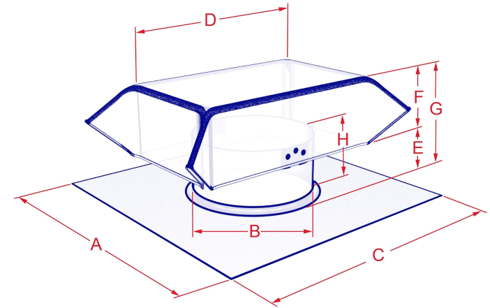
CRIMPED HOOD STYLE SIZES: 14"
