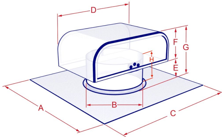
3 PIECE HOOD STYLE SIZES: 5", 7", 10" & 12"
