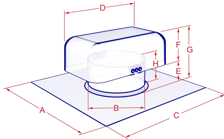
DRAWN HOOD STYLE SIZES: 3", 4", 6" & 8"
